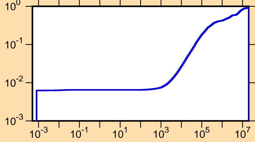
\mu vs. E for ^{108}\text{Sn}(\text{mt251})
