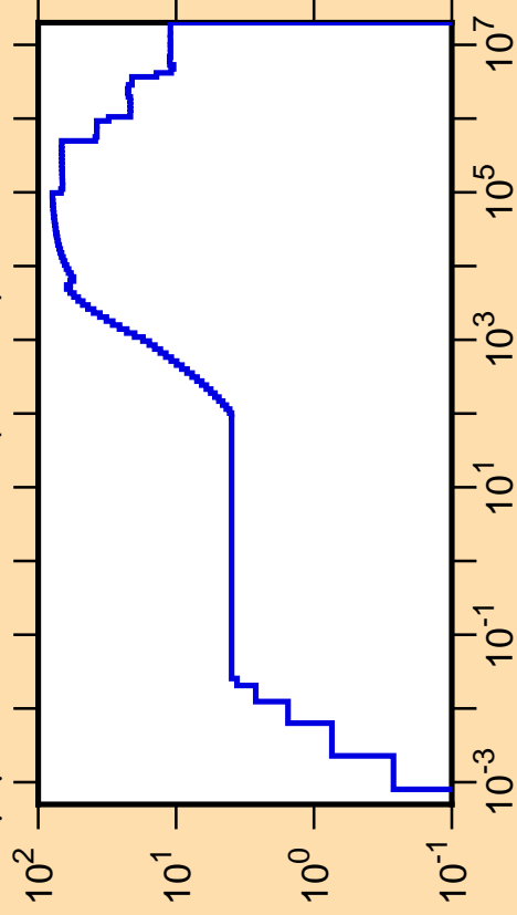
\Delta\mu/\mu vs. E for ^{108}\text{Sn}(\text{mt251})
