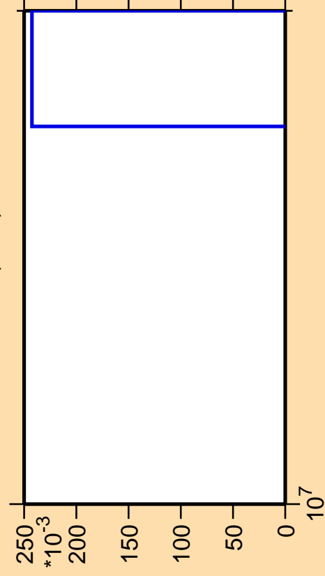
\Delta\sigma/\sigma vs. E for ^{108}\text{Sn}(n,nt)
