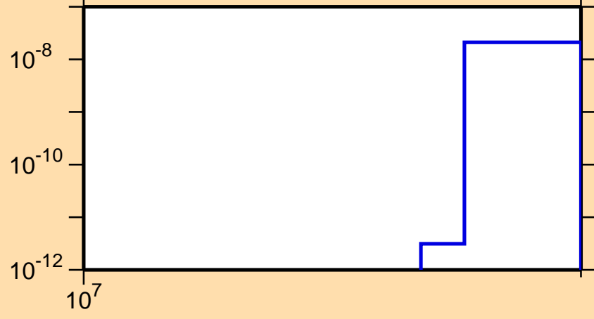
\sigma vs. E for ^{108}\text{Sn}(n,2n\alpha)
