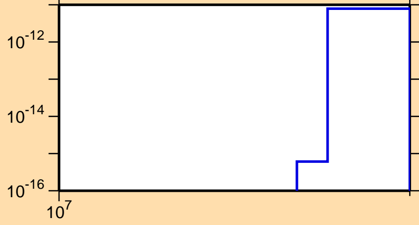
\sigma vs. E for ^{108}\text{Sn}(\text{mt } 34)
