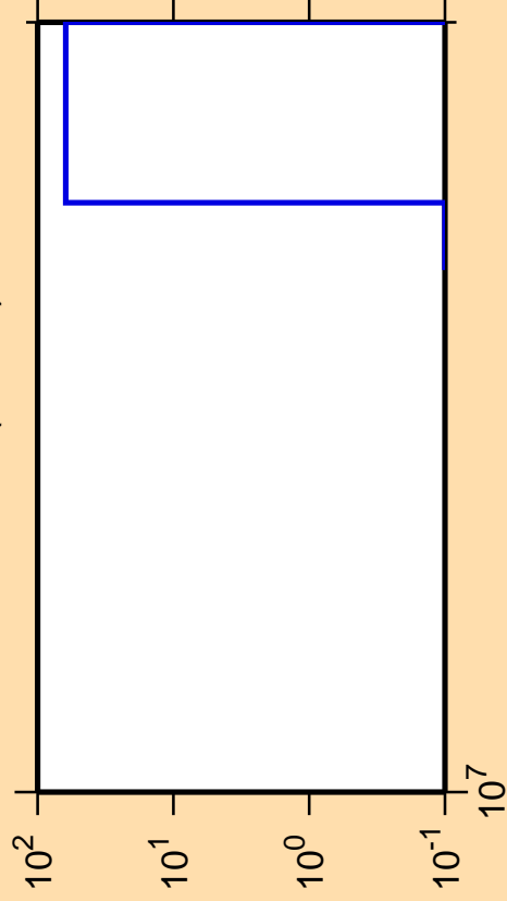
\Delta\sigma/\sigma vs. E for ^{108}\text{Sn}(\text{mt } 34)
