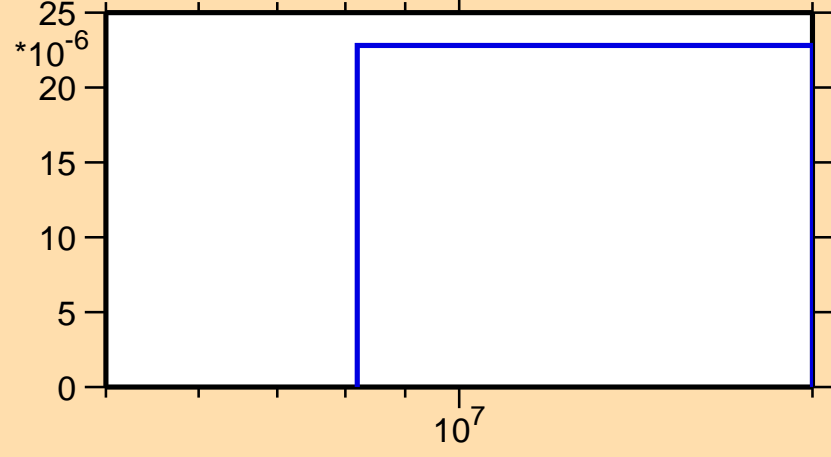
\sigma vs. E for ^{108}\text{Sn}(n,t)
