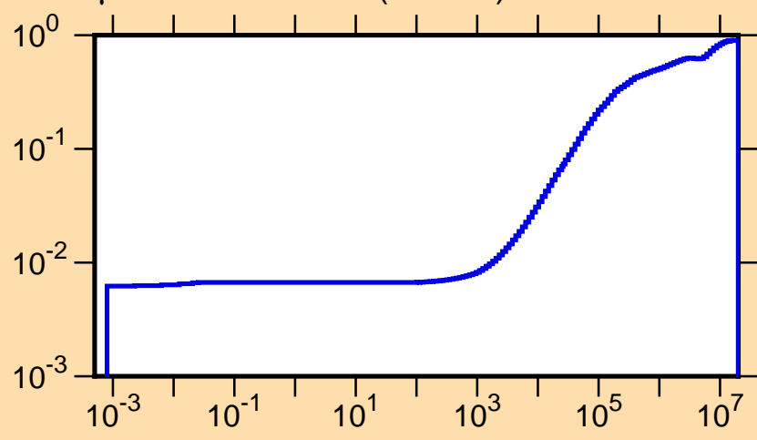
\mu vs. E for ^{109}\text{Sn}(\text{mt251})
