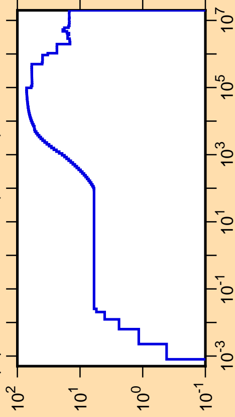
\Delta\mu/\mu vs. E for ^{109}\text{Sn}(\text{mt251})
