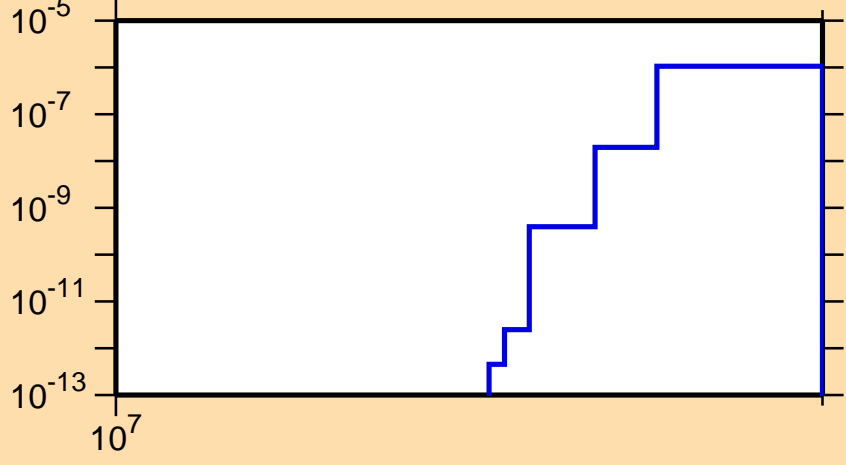
\sigma vs. E for ^{109}\text{Sn}(n,\text{pt})
