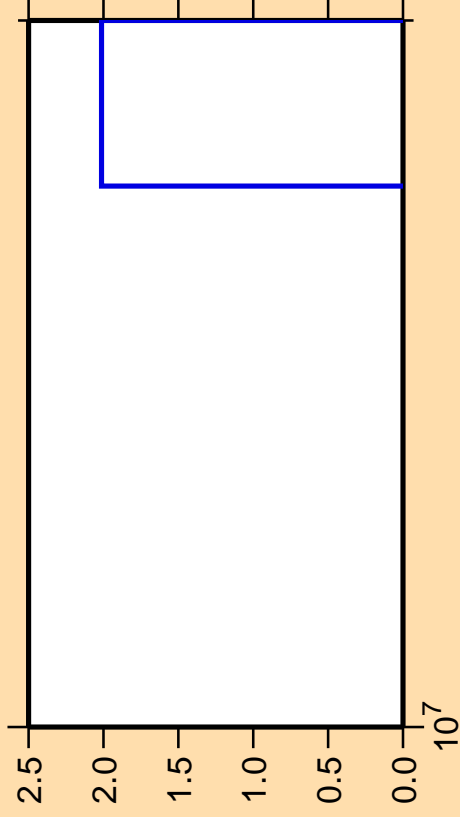
\Delta\sigma/\sigma vs. E for ^{109}\text{Sn}(n,nt)
