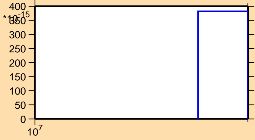
\sigma vs. E for ^{109}\text{Sn}(n,nt)
