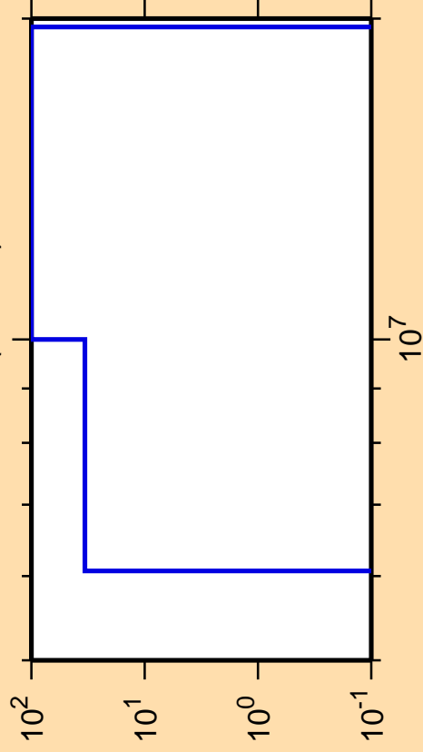
\Delta\sigma/\sigma vs. E for ^{109}\text{Sn}(n,\text{He3})
