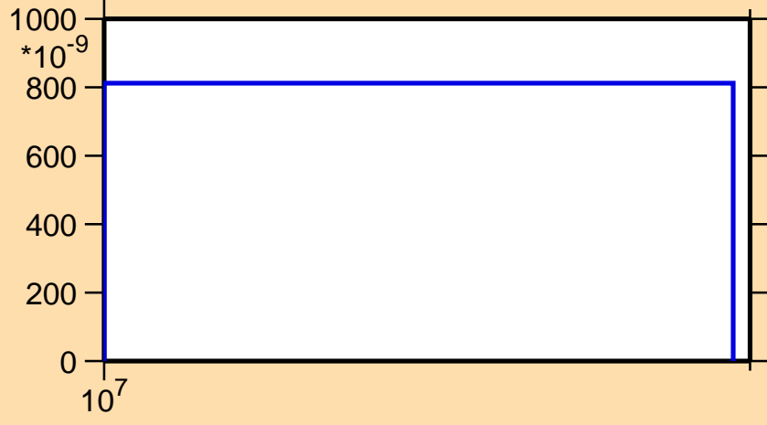
\sigma vs. E for ^{109}\text{Sn}(n,\text{nd})
