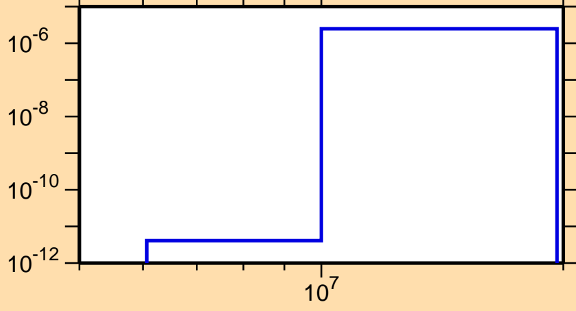
\sigma vs. E for ^{109}\text{Sn}(n,\text{He3})
