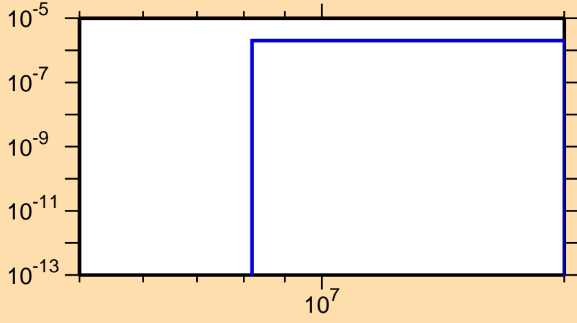
\sigma vs. E for ^{109}\text{Sn}(n,\text{He3})
