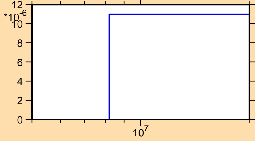
\sigma vs. E for ^{109}\text{Sn}(n,2np)
