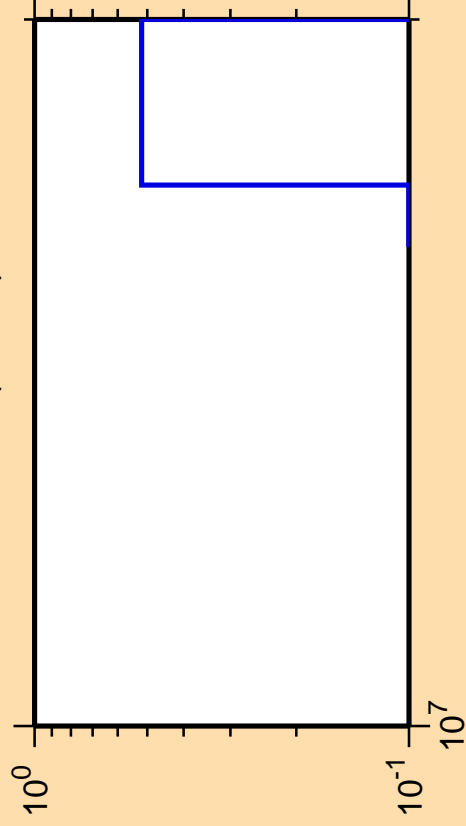
\Delta\sigma/\sigma vs. E for ^{110}\text{Sn} (mt 34)
