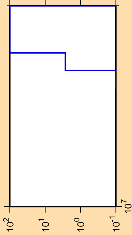
\Delta\sigma/\sigma vs. E for ^{110}\text{Sn}(n,nd)
