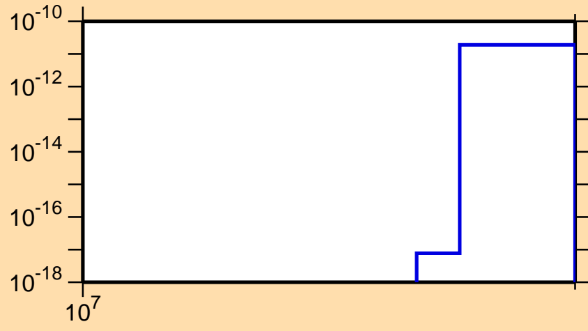
\sigma vs. E for ^{110}\text{Sn}(n,\text{pt})
