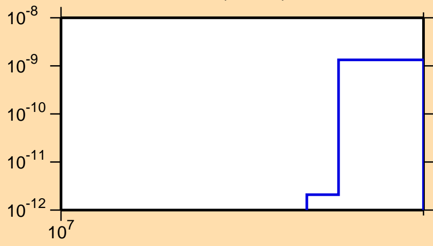
\sigma vs. E for ^{110}\text{Sn} (mt 45)
