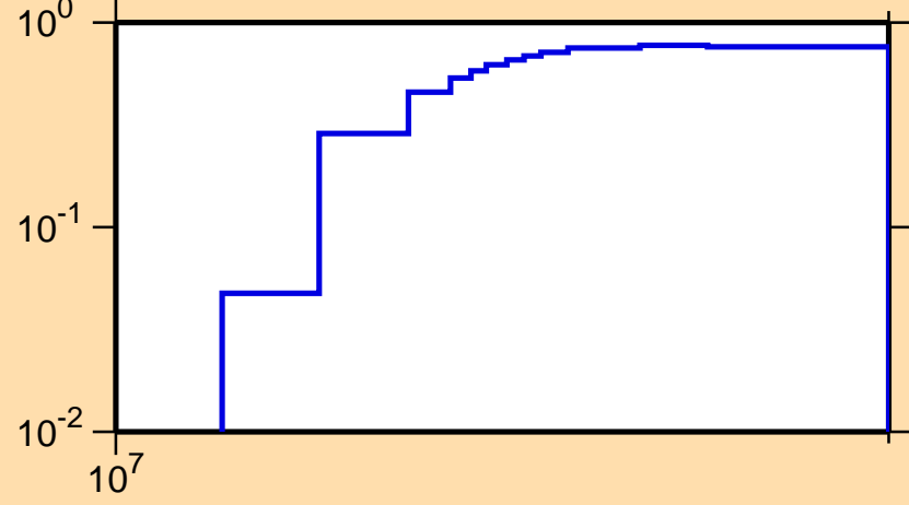
\sigma vs. E for ^{110}\text{Sn}(n,2n)
