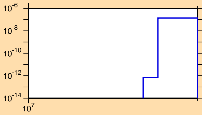
\sigma vs. E for ^{110}\text{Sn}(n,nd)
