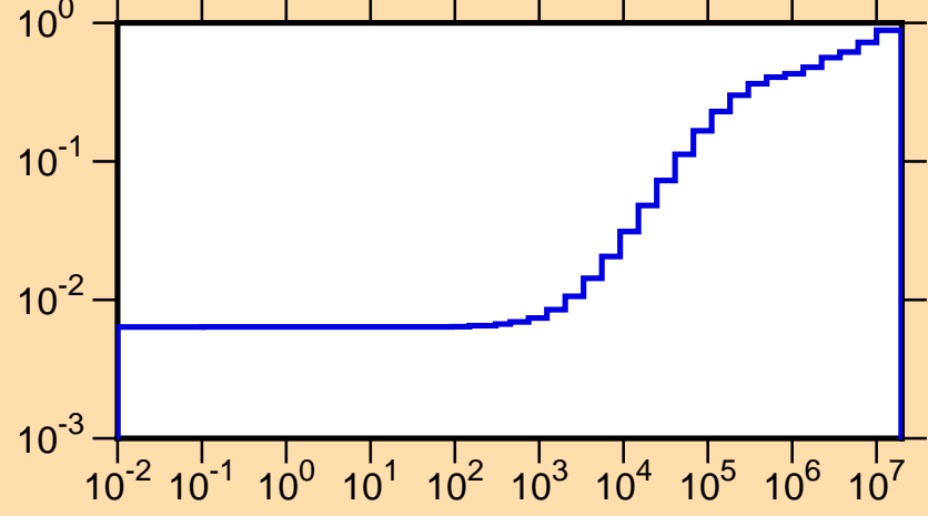
\mu vs. E for ^{110}\text{Sn}(\text{mt251})
