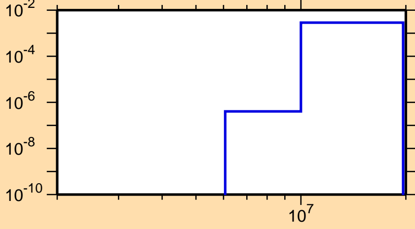
\sigma vs. E for ^{110}\text{Sn}(n,d)
