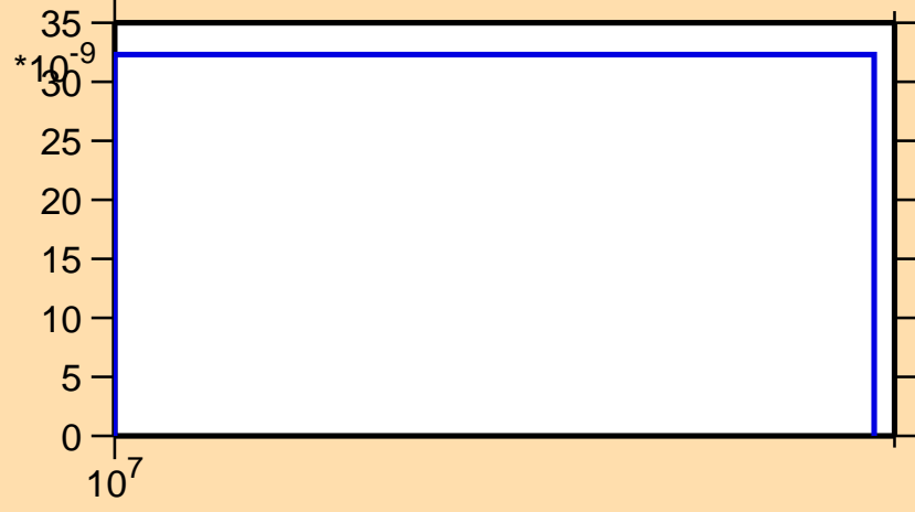
\sigma vs. E for ^{110}\text{Sn}(n,pd)
