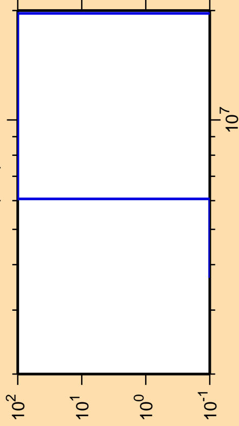
\Delta\sigma/\sigma vs. E for ^{110}\text{Sn}(n,d)
