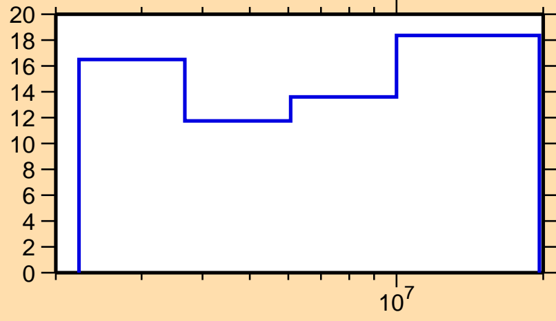
\Delta\sigma/\sigma vs. E for ^{110}\text{Sn}(n,n\text{cont.})
