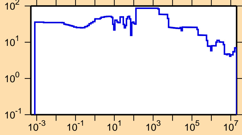
\Delta\sigma/\sigma vs. E for ^{111}\text{Sn}(n,\text{tot.})
