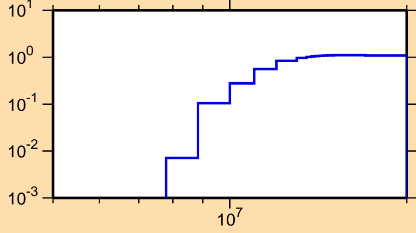
\sigma vs. E for ^{111}\text{Sn}(n,2n)
