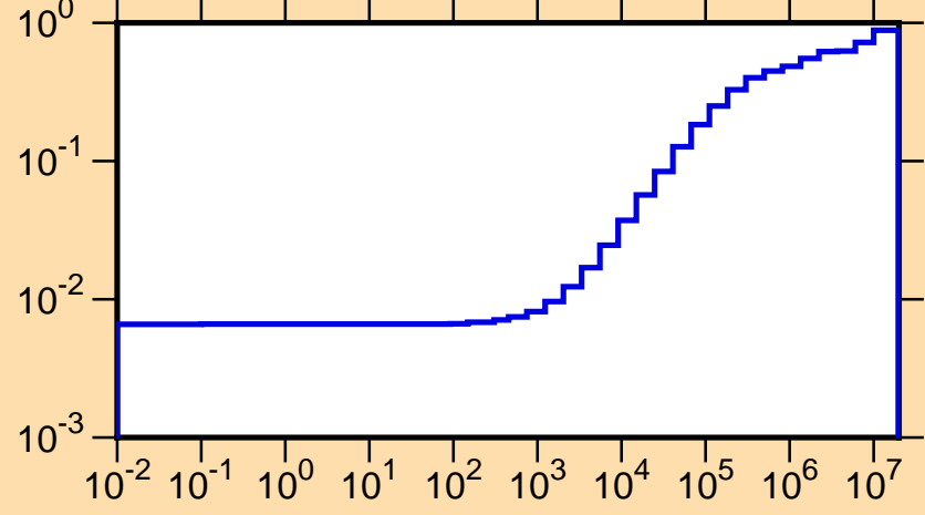
\mu vs. E for ^{111}\text{Sn}(\text{mt251})
