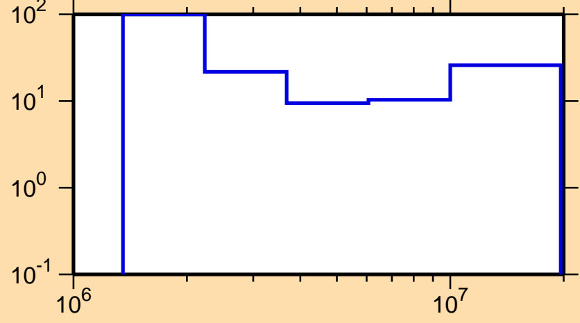
\Delta\sigma/\sigma vs. E for ^{111}\text{Sn}(n,ncont.)
