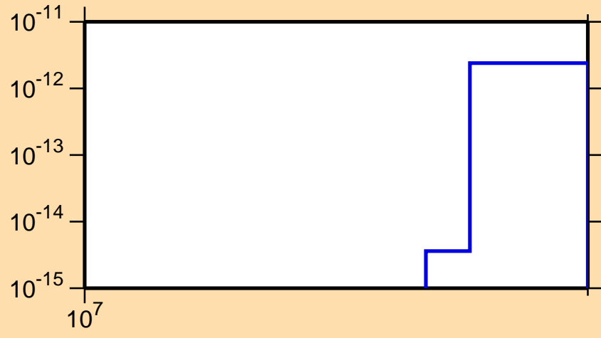
\sigma vs. E for ^{112}\text{Sn}(\text{mt117})
