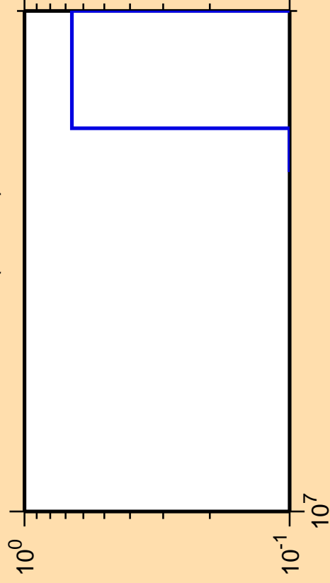
\Delta\sigma/\sigma vs. E for ^{112}\text{Sn}(\text{mt } 45)
