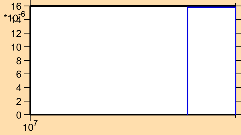
\sigma vs. E for ^{112}\text{Sn}(n,3n)
