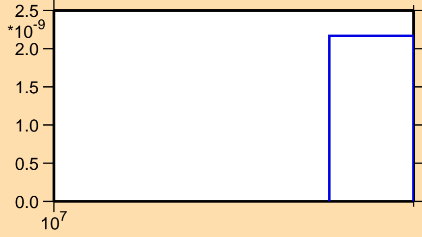
\sigma vs. E for ^{112}\text{Sn}(n,2np)
