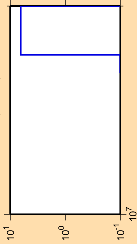
\Delta\sigma/\sigma vs. E for ^{112}\text{Sn}(\text{mt117})
