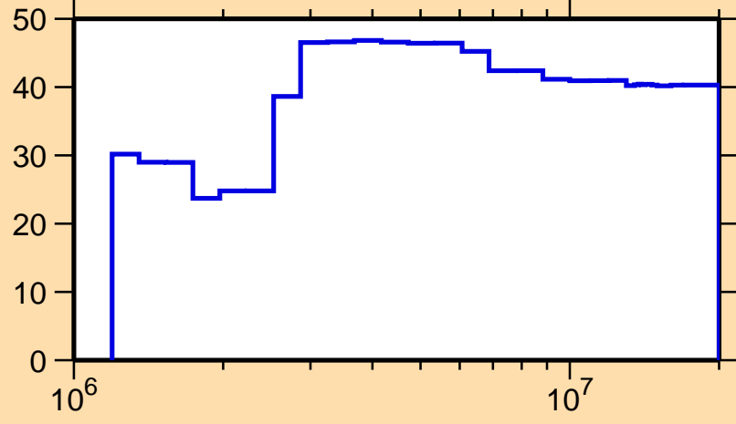
\Delta\sigma/\sigma vs. E for ^{112}\text{Sn}(n,n_1)
