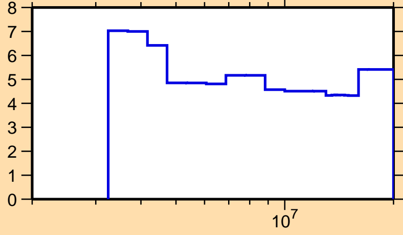
\Delta\sigma/\sigma vs. E for ^{112}\text{Sn}(n,n\text{nonel.})
