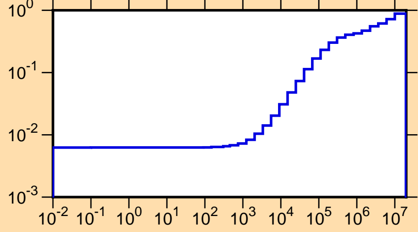
\mu vs. E for ^{112}\text{Sn}(\text{mt251})
