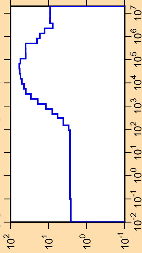
\Delta\mu/\mu vs. E for ^{112}\text{Sn}(\text{mt251})
