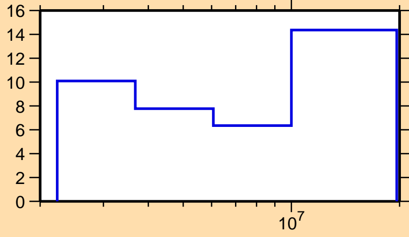
\Delta\sigma/\sigma vs. E for ^{112}\text{Sn}(n,n\text{cont.})
