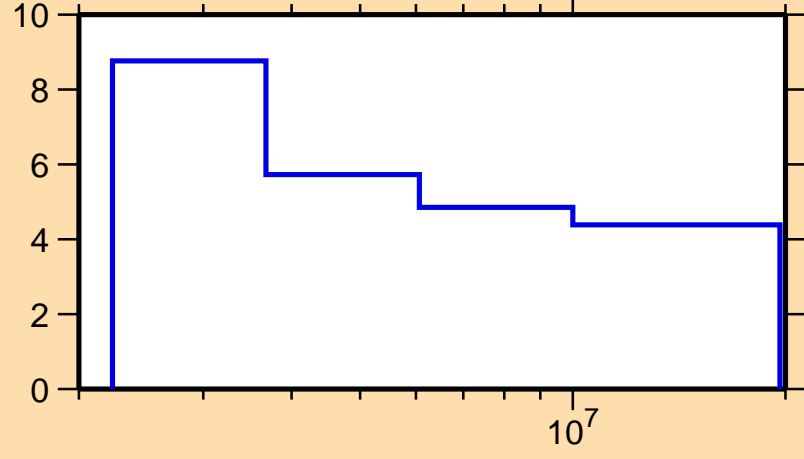
\Delta\sigma/\sigma vs. E for ^{112}\text{Sn}(n,\text{nonel.})
