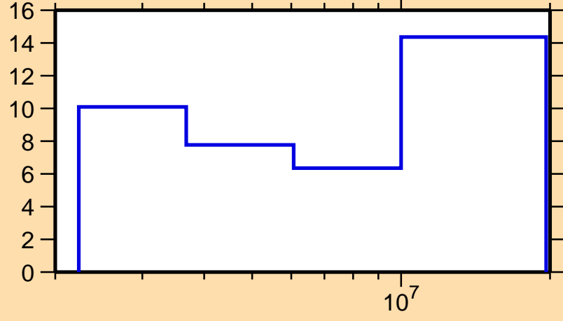
\Delta\sigma/\sigma vs. E for ^{112}\text{Sn}(n,ncont.)
