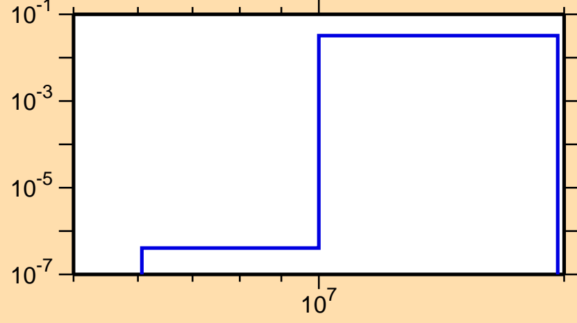
\sigma vs. E for ^{112}\text{Sn}(n,np)
