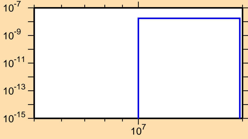
\sigma vs. E for ^{112}\text{Sn}(n,\text{He3})
