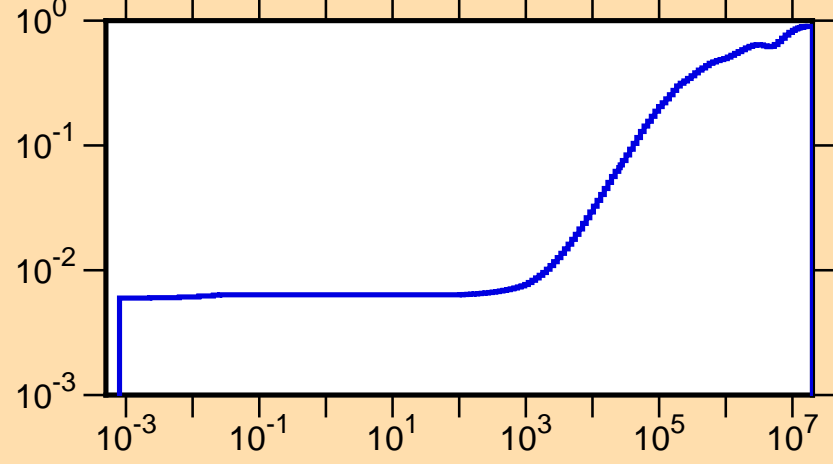
\mu vs. E for ^{113}\text{Sn}(\text{mt251})
