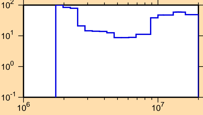
\Delta\sigma/\sigma vs. E for ^{113}\text{Sn}(n,n\text{cont.})
