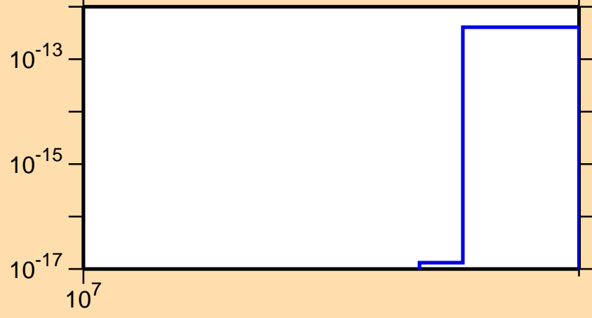
\sigma vs. E for ^{113}\text{Sn} (mt 34)
