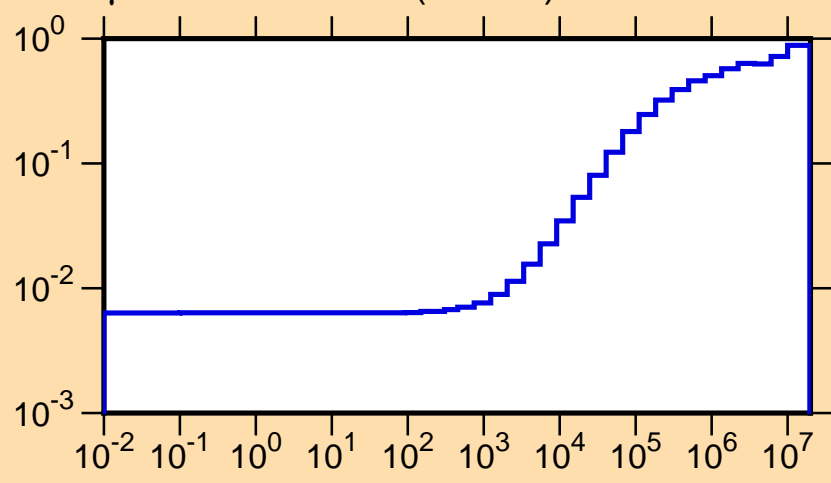
\mu vs. E for ^{113}\text{Sn}(\text{mt251})
