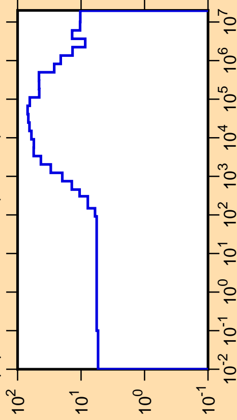
\Delta\mu/\mu vs. E for ^{113}\text{Sn}(\text{mt251})
