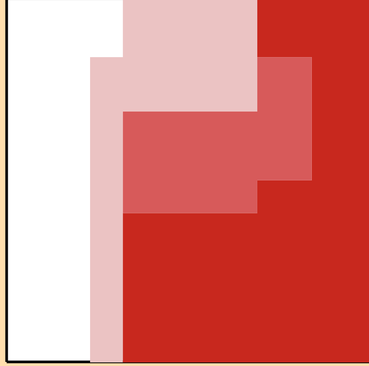
\Delta\sigma/\sigma vs. E for ^{113}\text{Sn}(n,2n)
