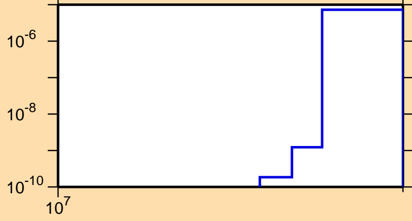
\sigma vs. E for ^{113}\text{Sn}(n,2np)
