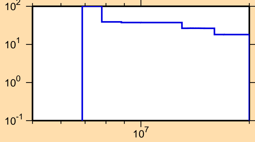
\Delta\sigma/\sigma vs. E for ^{113}\text{Sn}(n,2n)
