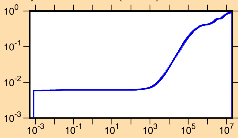
\mu vs. E for ^{114}\text{Sn}(\text{mt251})
