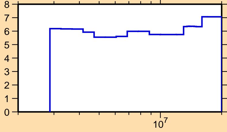
\Delta\sigma/\sigma vs. E for ^{114}\text{Sn}(n,\text{nonel.})
