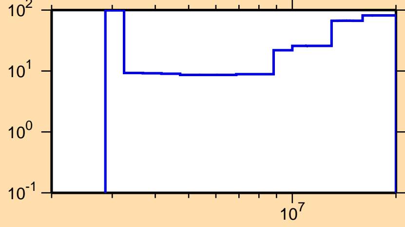
\Delta\sigma/\sigma vs. E for ^{114}\text{Sn}(n,n\text{cont.})
