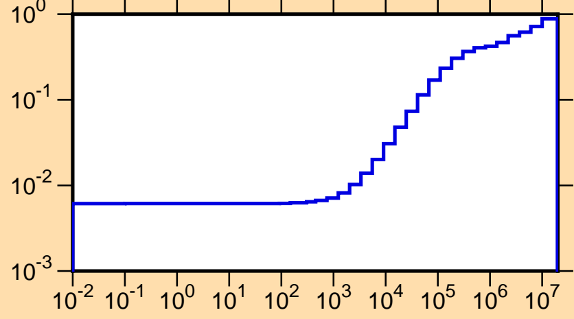
\mu vs. E for ^{114}\text{Sn}(\text{mt251})
