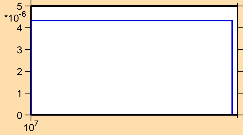
\sigma vs. E for ^{114}\text{Sn}(n,t)
