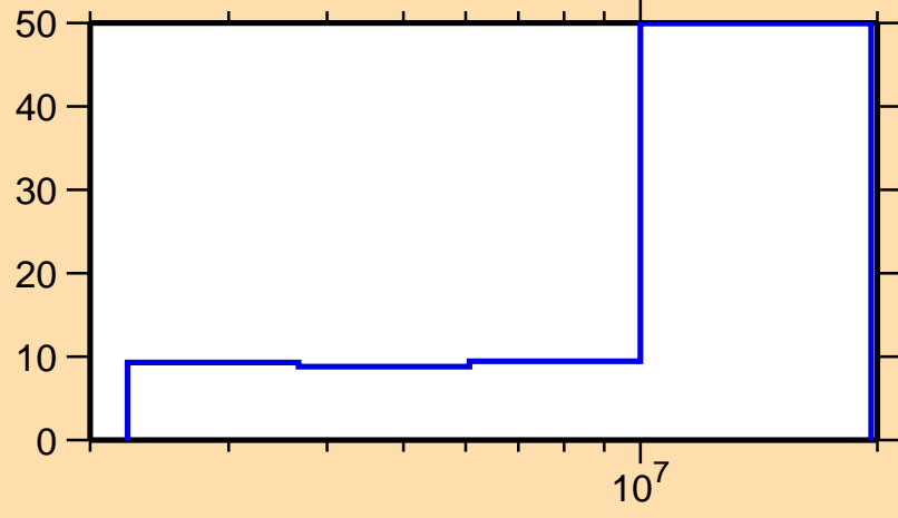
\Delta\sigma/\sigma vs. E for ^{114}\text{Sn}(n,n\text{cont.})
