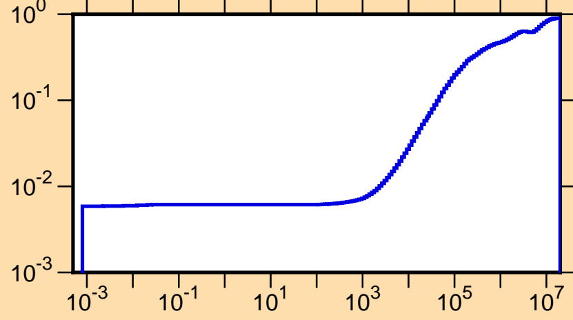
\mu vs. E for ^{115}\text{Sn}(\text{mt251})
