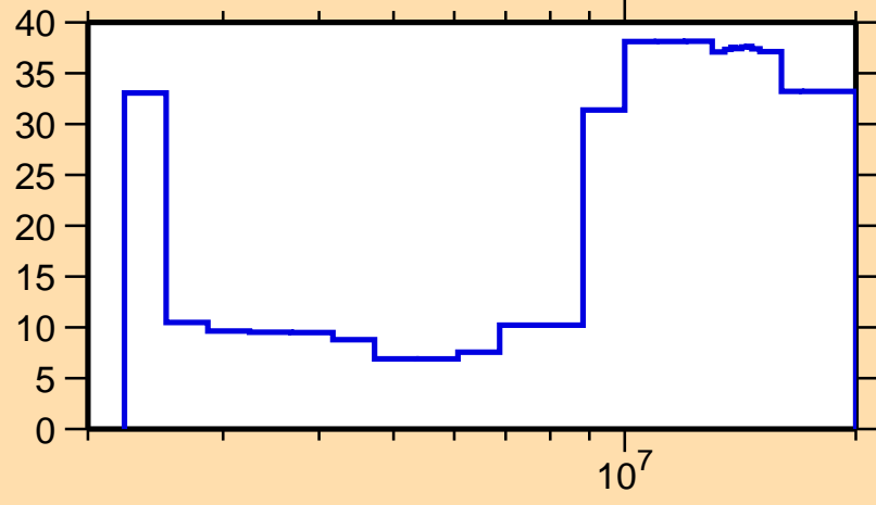
\Delta\sigma/\sigma vs. E for ^{115}\text{Sn}(n,ncont.)
