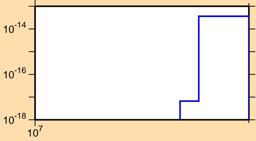
\sigma vs. E for ^{115}\text{Sn}(n,\text{pt})
