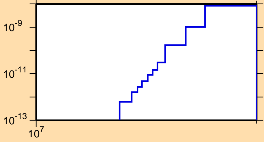
\sigma vs. E for ^{115}\text{Sn}(n,p\alpha)
