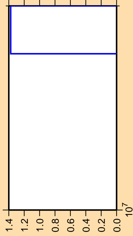
\Delta\sigma/\sigma vs. E for ^{115}\text{Sn}(n,nt)
