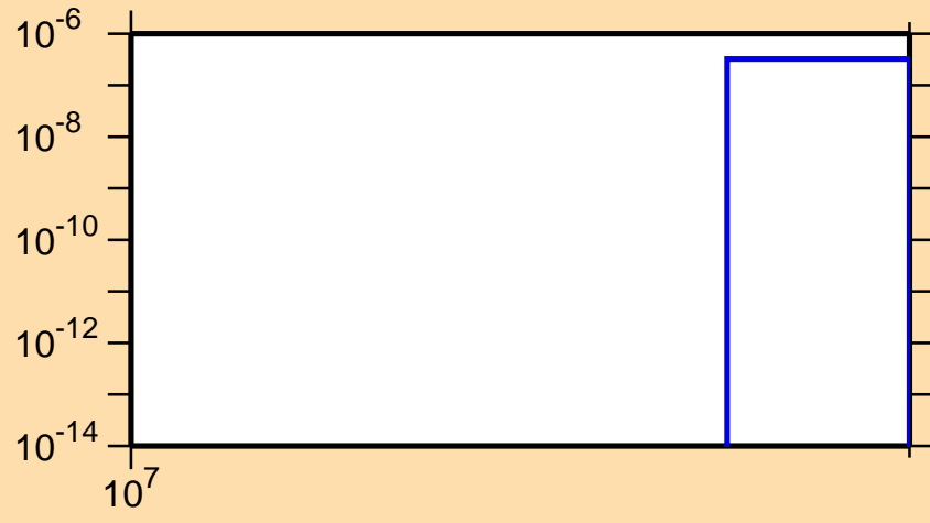
\sigma vs. E for ^{115}\text{Sn}(n,2np)
