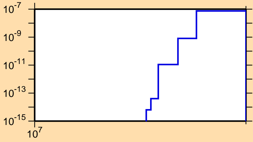
\sigma vs. E for ^{115}\text{Sn}(n,2n\alpha)
