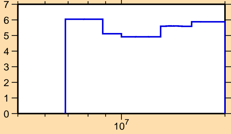
\Delta\sigma/\sigma vs. E for ^{115}\text{Sn}(n,\text{nonel.})
