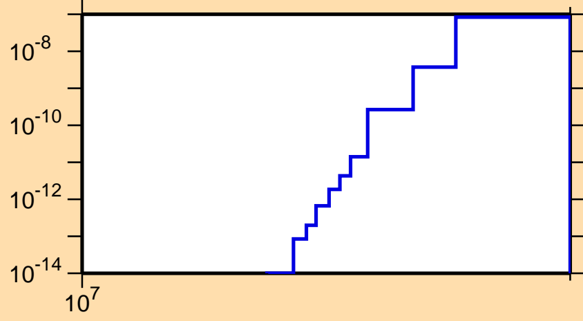
\sigma vs. E for ^{115}\text{Sn}(n,\text{He3})
