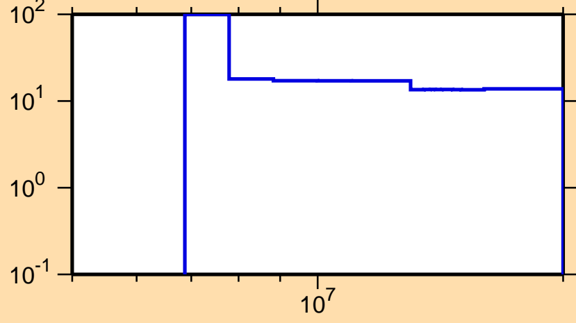
\Delta\sigma/\sigma vs. E for ^{115}\text{Sn}(n,2n)
