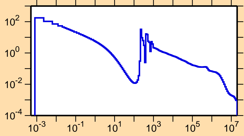
\sigma vs. E for ^{115}\text{Sn}(n,\gamma)
