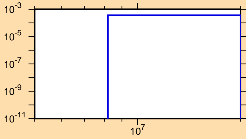
\sigma vs. E for ^{115}\text{Sn}(n,n\alpha)
