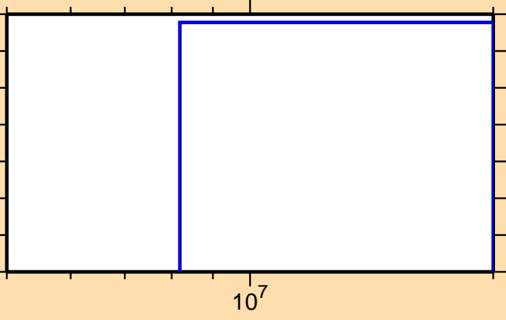
\sigma vs. E for ^{115}\text{Sn}(n,\text{nd})
