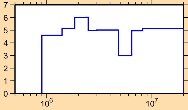
\Delta\sigma/\sigma vs. E for ^{115}\text{Sn}(n,el.)
