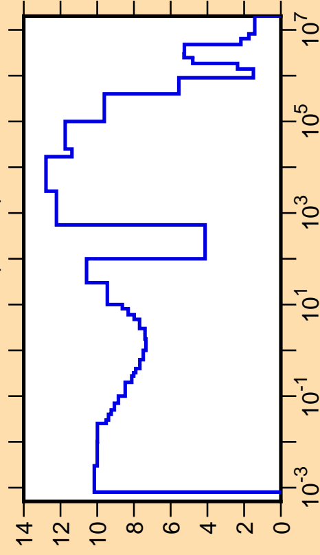
\Delta\sigma/\sigma vs. E for ^{115}\text{Sn}(n,\text{tot.})
