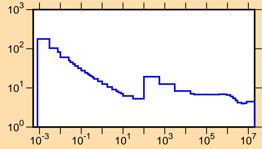
\sigma vs. E for ^{115}\text{Sn}(n,\text{tot.})
