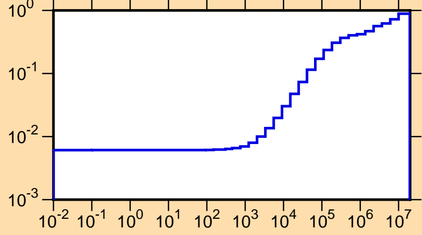
\mu vs. E for ^{116}\text{Sn}(\text{mt251})
