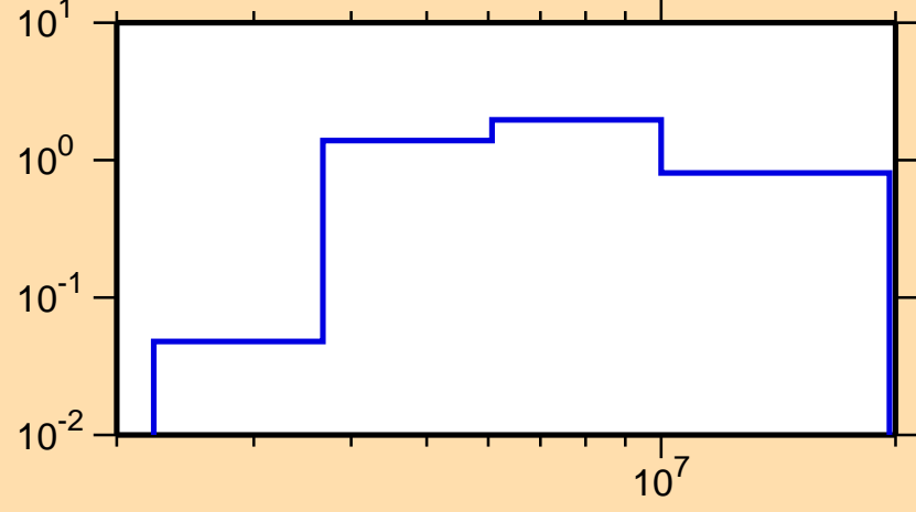
\sigma vs. E for ^{116}\text{Sn}(n,n\text{cont.})
