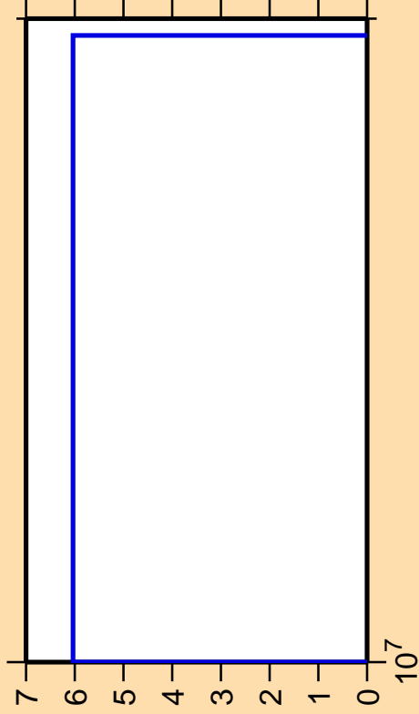
\Delta\sigma/\sigma vs. E for ^{116}\text{Sn}(n,nd)
