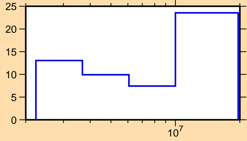
\Delta\sigma/\sigma vs. E for ^{116}\text{Sn}(n,n\text{cont.})
