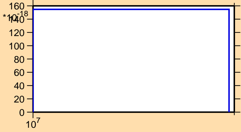
\sigma vs. E for ^{116}\text{Sn}(n,\text{pd})
