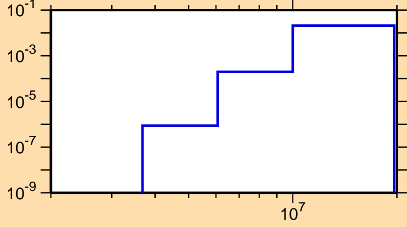
\sigma vs. E for ^{116}\text{Sn}(n,p)
