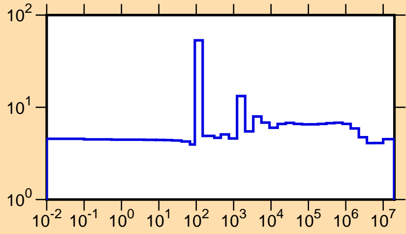
\sigma vs. E for ^{116}\text{Sn}(n,\text{tot.})
