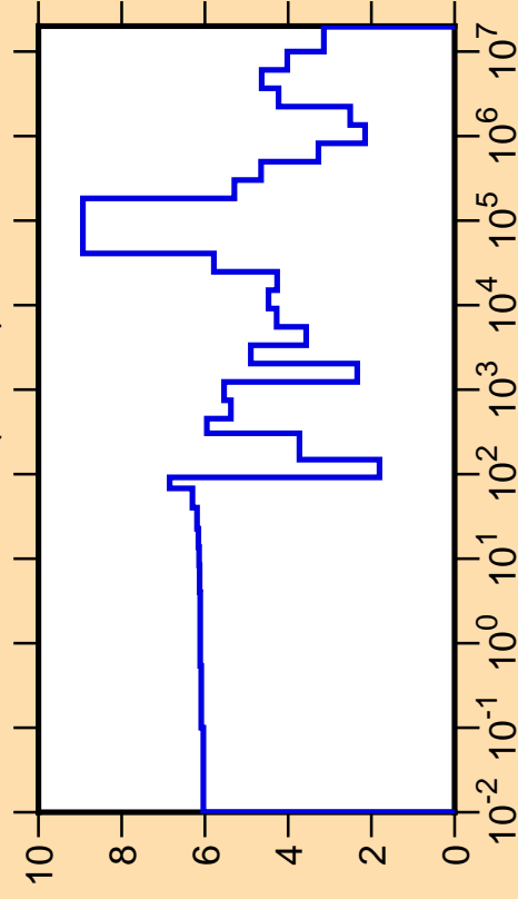
\Delta\sigma/\sigma vs. E for ^{116}\text{Sn}(n,\text{tot.})
