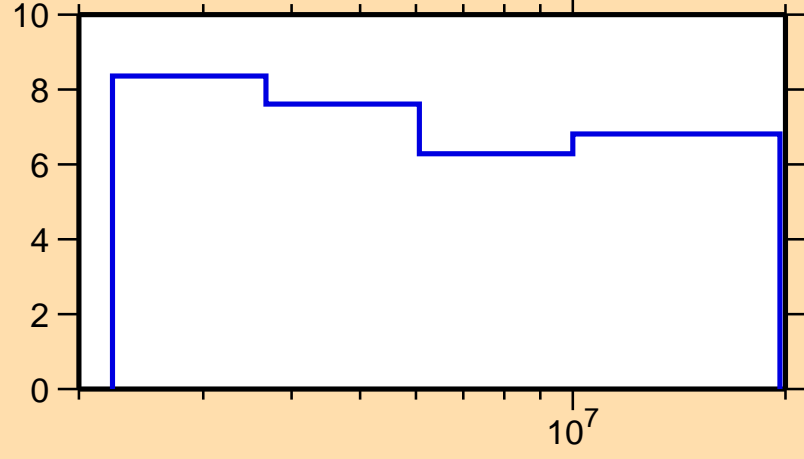
\Delta\sigma/\sigma vs. E for ^{116}\text{Sn}(n,n_{\text{nonel.}})
