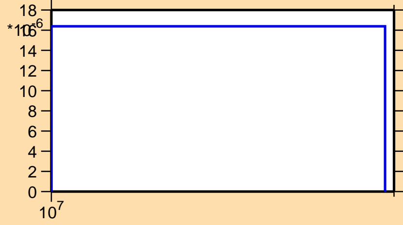
\sigma vs. E for ^{116}\text{Sn}(n,3n)
