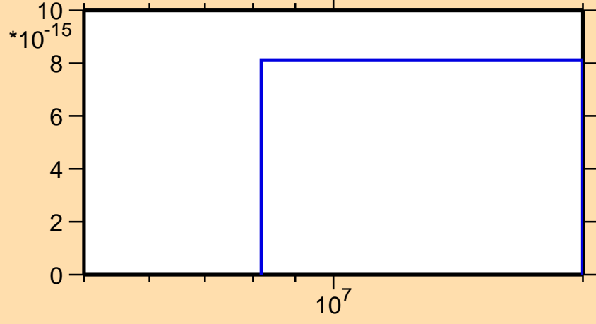
\sigma vs. E for ^{116}\text{Sn}(n,2np)
