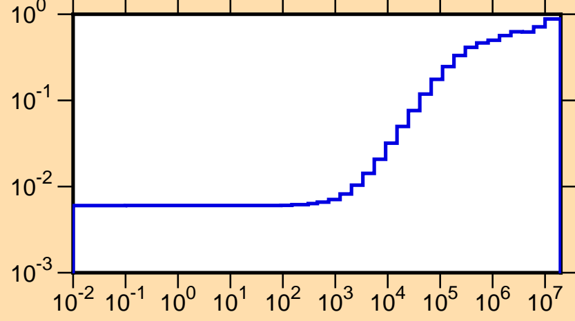
\mu vs. E for ^{117}\text{Sn}(\text{mt251})
