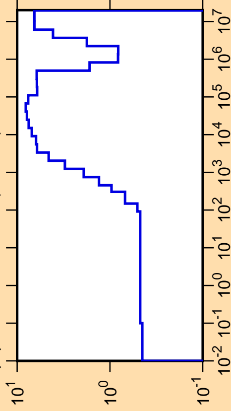
\Delta\mu/\mu vs. E for ^{117}\text{Sn}(\text{mt251})
