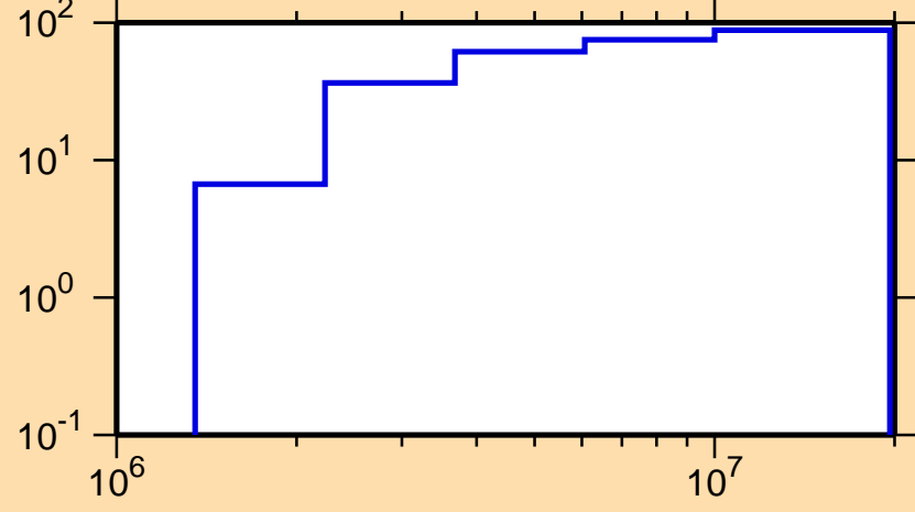
\Delta\sigma/\sigma vs. E for ^{117}\text{Sn}(n,n_1)
