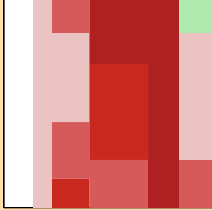
\Delta\sigma/\sigma vs. E for ^{117}\text{Sn}(n,2n)
