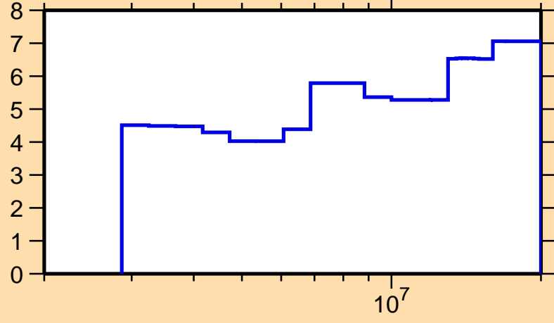
\Delta\sigma/\sigma vs. E for ^{118}\text{Sn}(n,n_{\text{inel}}) .
