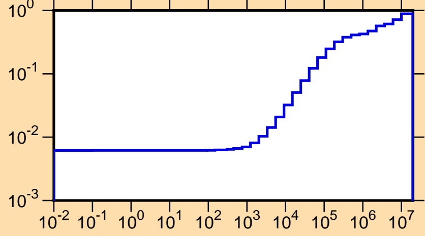
\mu vs. E for ^{118}\text{Sn}(\text{mt251})
