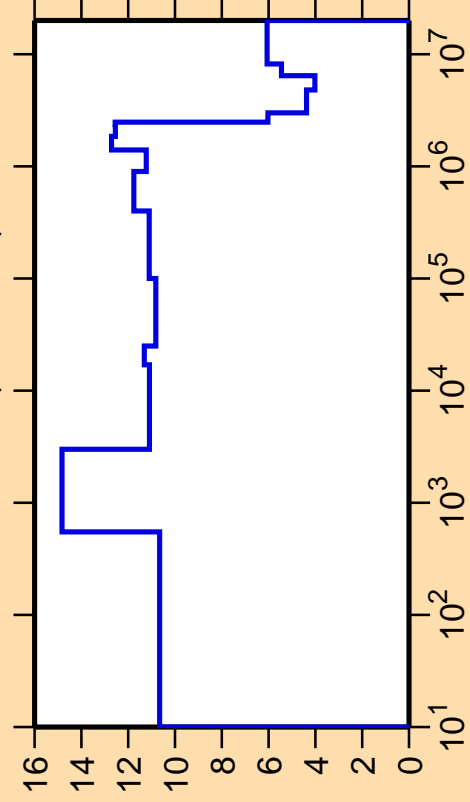
\Delta\sigma/\sigma vs. E for ^{118}\text{Sn}(n,\text{nonel.})
