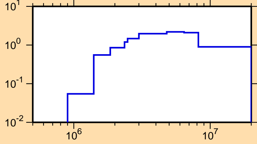
\sigma vs. E for ^{118}\text{Sn}(n,\text{inel.})
