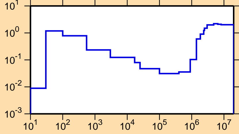
\sigma vs. E for ^{118}\text{Sn}(n,\text{nonel.})
