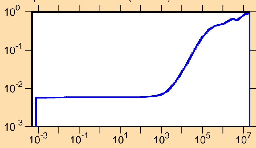
\mu vs. E for ^{119}\text{Sn}(\text{mt251})
