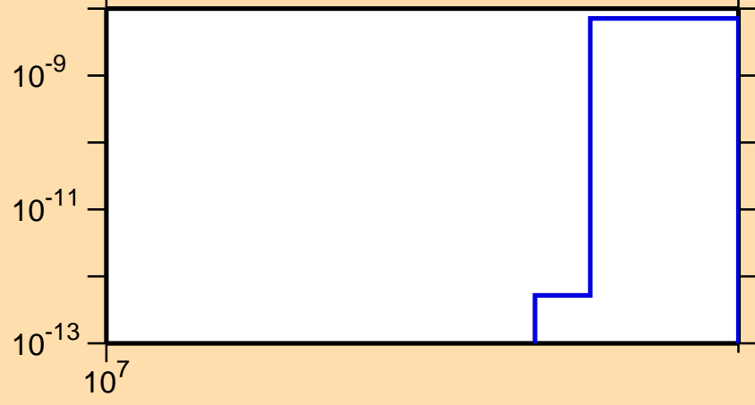
\sigma vs. E for ^{119}\text{Sn}(n,2np)
