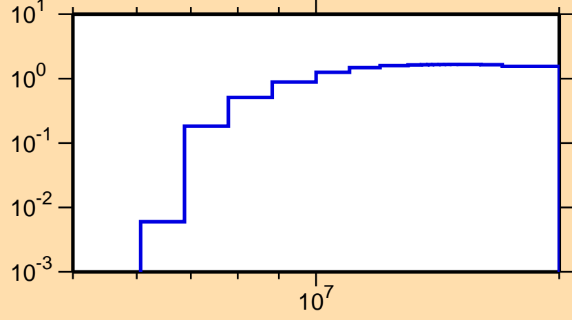
\sigma vs. E for ^{119}\text{Sn}(n,2n)
