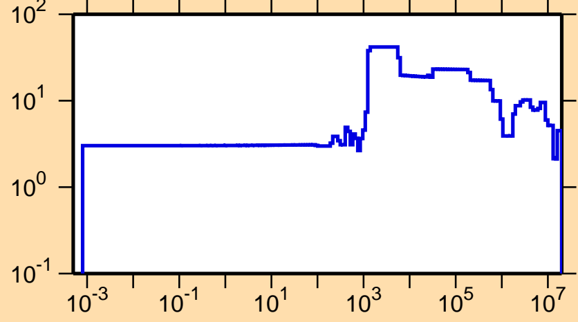
\Delta\sigma/\sigma vs. E for ^{119}\text{Sn}(n,\text{el.})
