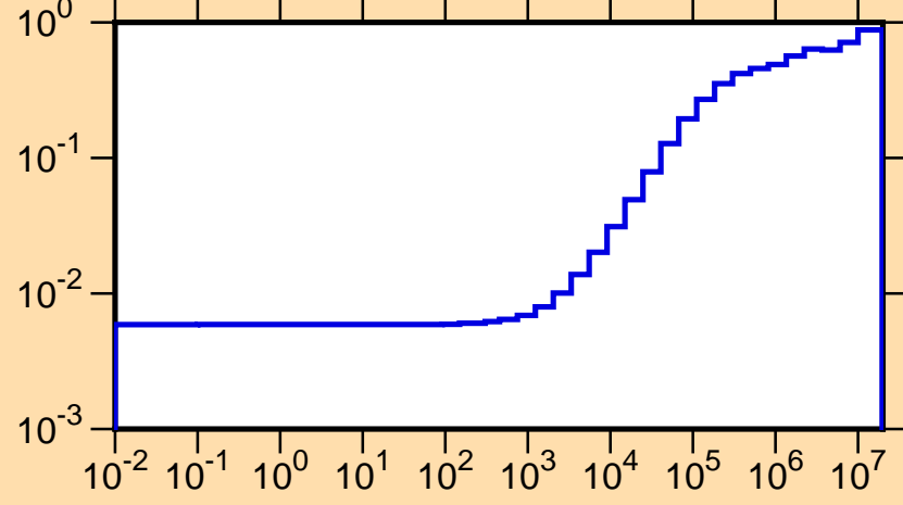
\mu vs. E for ^{119}\text{Sn}(\text{mt251})
