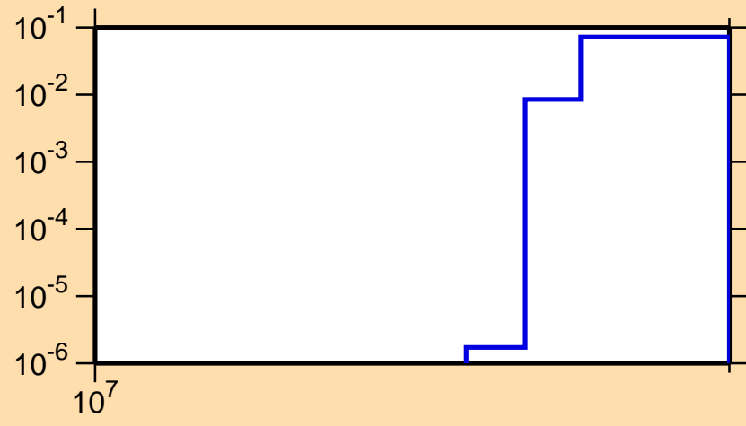
\sigma vs. E for ^{119}\text{Sn}(n,3n)
