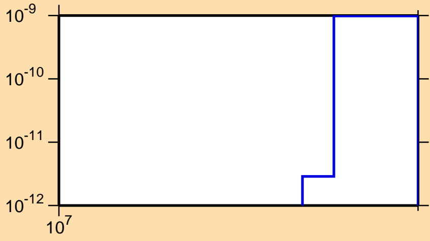
\sigma vs. E for ^{119}\text{Sn}(n,2n\alpha)
