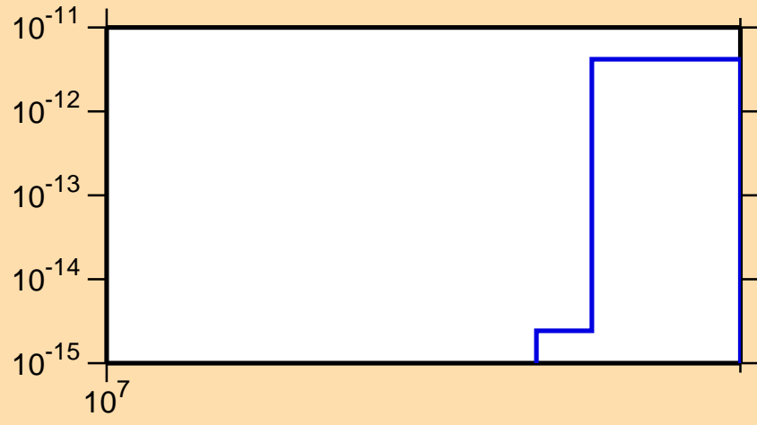
\sigma vs. E for ^{119}\text{Sn}(n,\text{He3})
