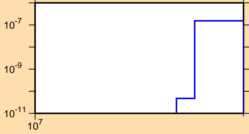
\sigma vs. E for ^{119}\text{Sn}(n,\text{nd})
