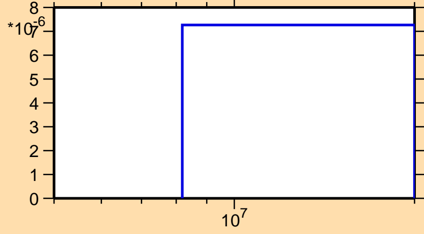
\sigma vs. E for ^{119}\text{Sn}(n,t)
