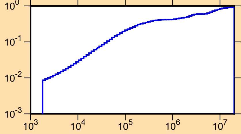
\mu vs. E for ^{120}\text{Sn}(\text{mt251})
