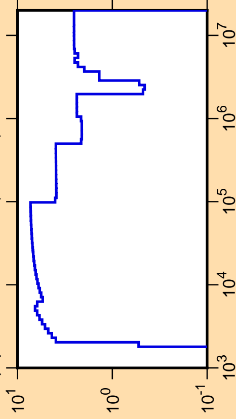
\Delta\mu/\mu vs. E for ^{120}\text{Sn}(\text{mt251})
