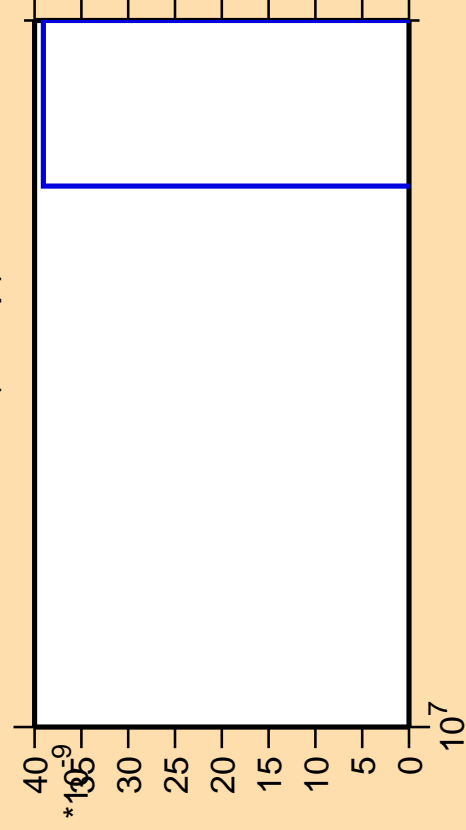
\Delta\sigma/\sigma vs. E for ^{120}\text{Sn}(n,2np)
