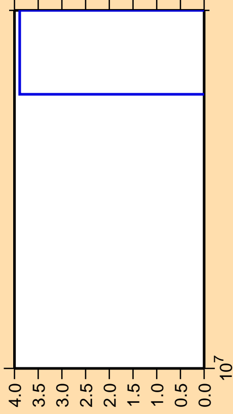
\Delta\sigma/\sigma vs. E for ^{120}\text{Sn}(n,nd)
