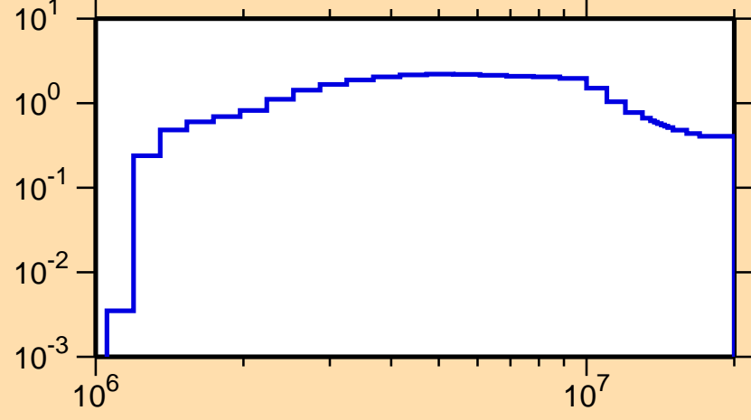
\sigma vs. E for ^{120}\text{Sn}(n,\text{inel.})
