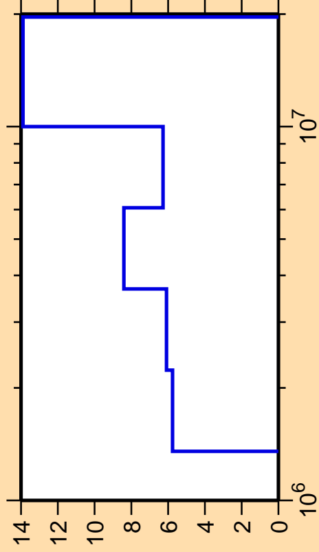
\Delta\sigma/\sigma vs. E for ^{120}\text{Sn}(n,n_3)
