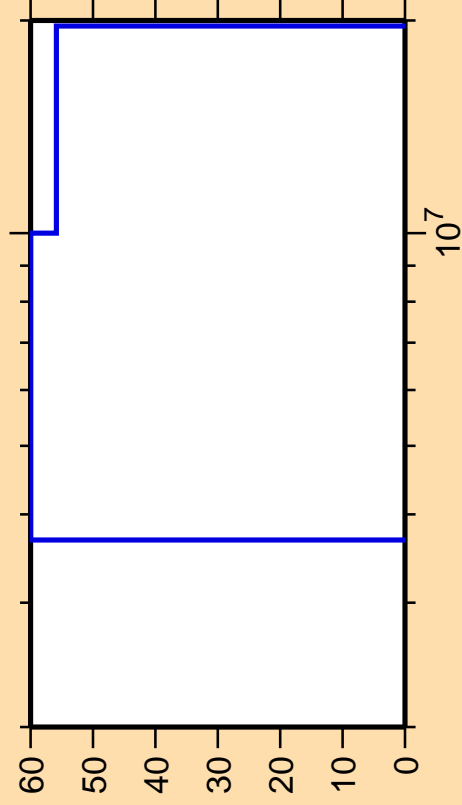
\Delta\sigma/\sigma vs. E for ^{120}\text{Sn}(n,\alpha)
