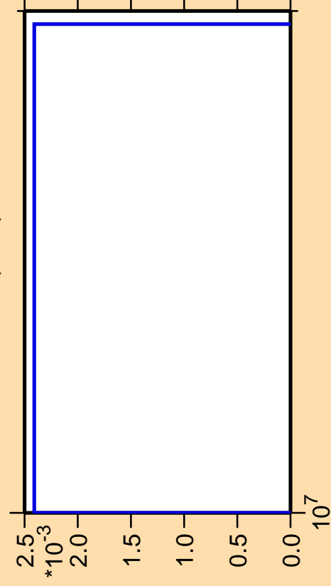
\Delta\sigma/\sigma vs. E for ^{120}\text{Sn}(n,nt)
