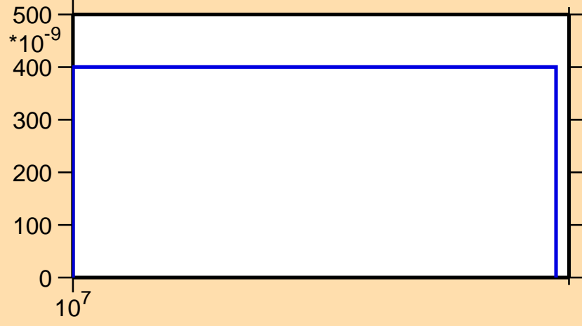
\sigma vs. E for ^{120}\text{Sn}(n,t)
