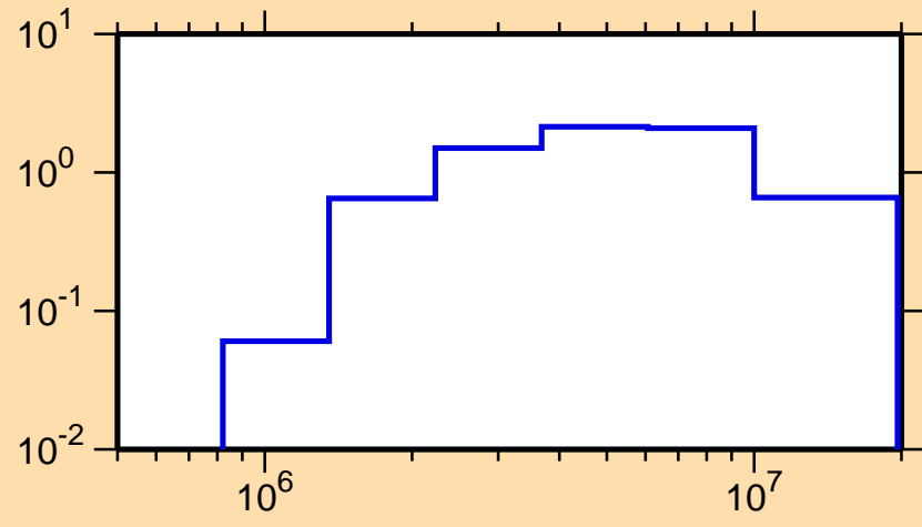
\sigma vs. E for ^{120}\text{Sn}(n,\text{inel.})
