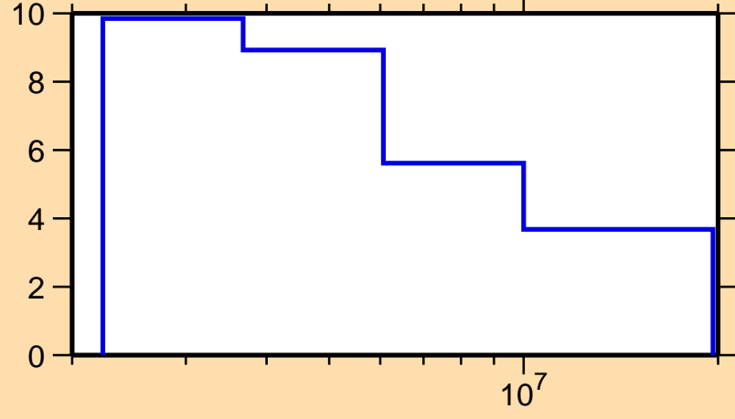
\Delta\sigma/\sigma vs. E for ^{120}\text{Sn}(n,n\text{onel.})
