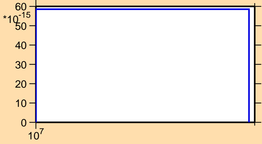
\sigma vs. E for ^{120}\text{Sn}(n,nd)
