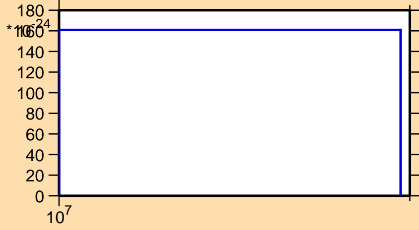
\sigma vs. E for ^{120}\text{Sn}(n,2np)
