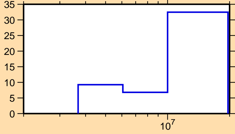
\Delta\sigma/\sigma vs. E for ^{120}\text{Sn}(n,ncont.)
