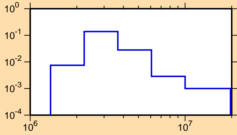
\sigma vs. E for ^{120}\text{Sn}(n,n_3)
