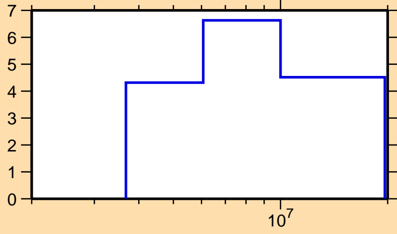
\Delta\sigma/\sigma vs. E for ^{120}\text{Sn}(n,el.)
