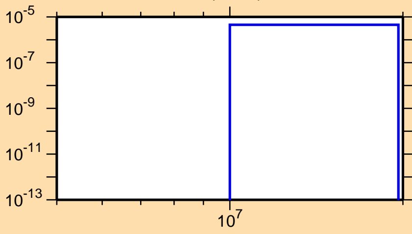
\sigma vs. E for ^{120}\text{Sn}(n,n\alpha)
