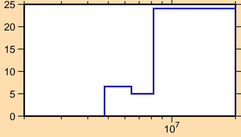
\Delta\sigma/\sigma vs. E for ^{120}\text{Sn}(n,n\text{cont.})
