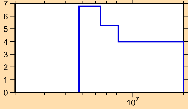
\Delta\sigma/\sigma vs. E for ^{120}\text{Sn}(n,\text{nonel.})
