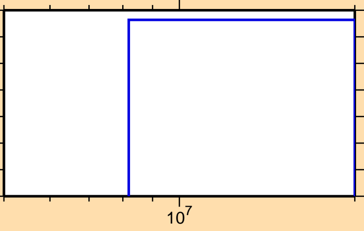
\sigma vs. E for ^{120}\text{Sn}(n,t)
