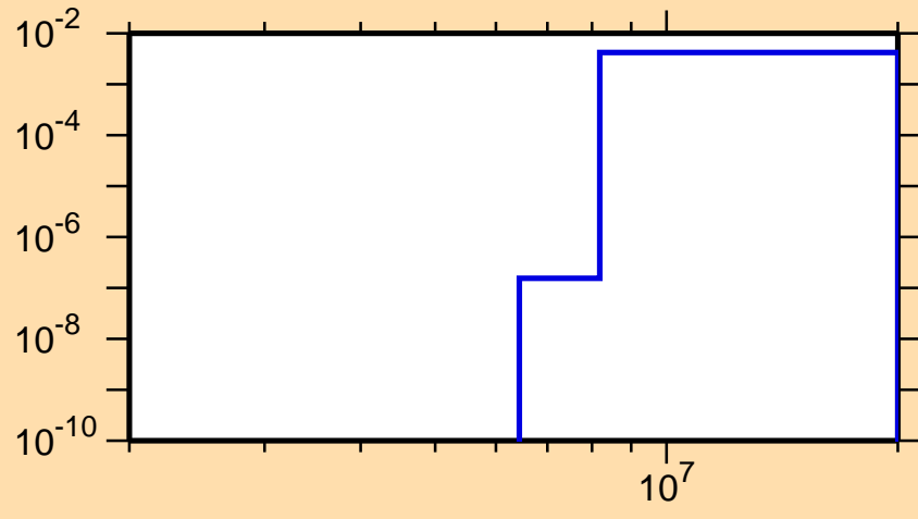
\sigma vs. E for ^{120}\text{Sn}(n,p)
