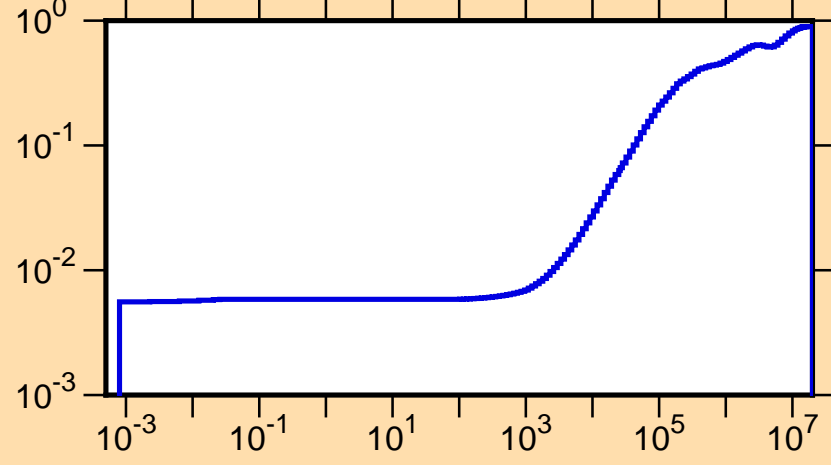
\mu vs. E for ^{121}\text{Sn}(\text{mt251})
