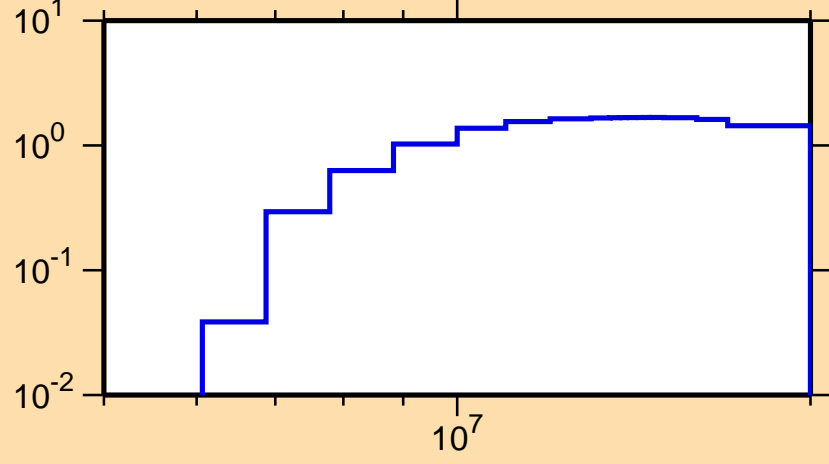
\sigma vs. E for ^{121}\text{Sn}(n,2n)
