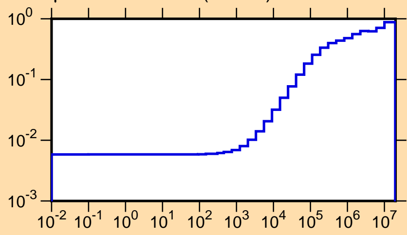
\mu vs. E for ^{121}\text{Sn}(\text{mt251})
