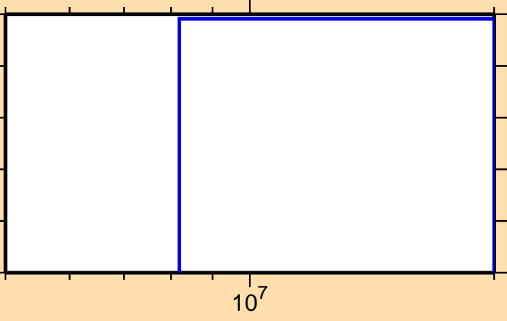
\sigma vs. E for ^{121}\text{Sn}(n,\text{nd})
