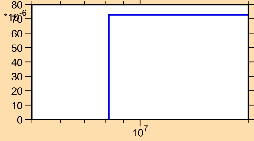
\sigma vs. E for ^{121}\text{Sn}(n,d)
