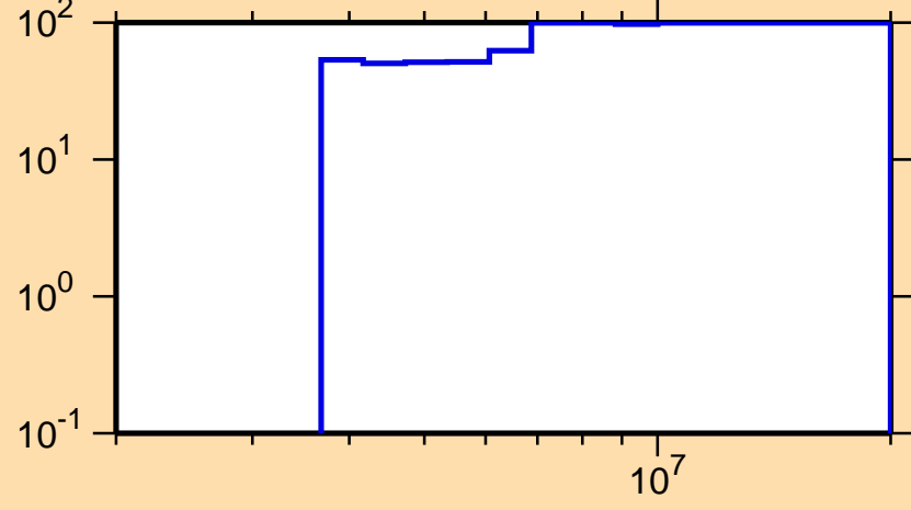
\Delta\sigma/\sigma vs. E for ^{123}\text{Sn}(n,n_1)
