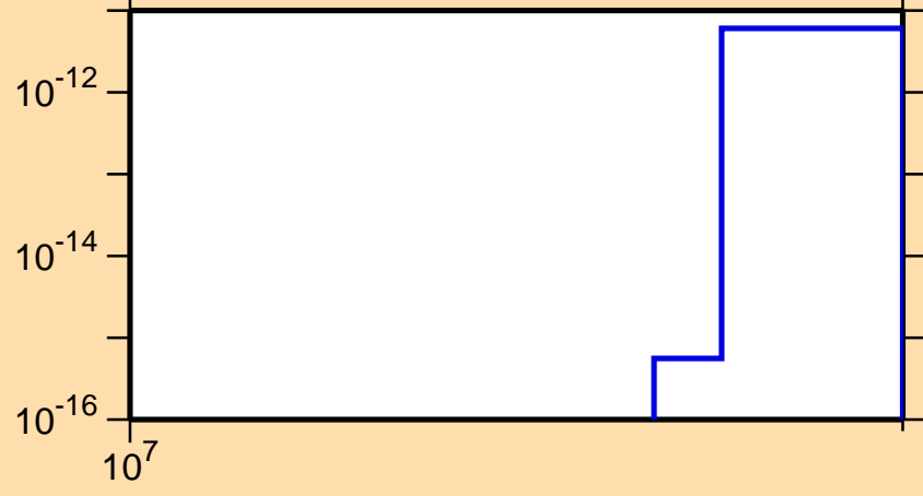
\sigma vs. E for ^{123}\text{Sn}(n,2n\alpha)
